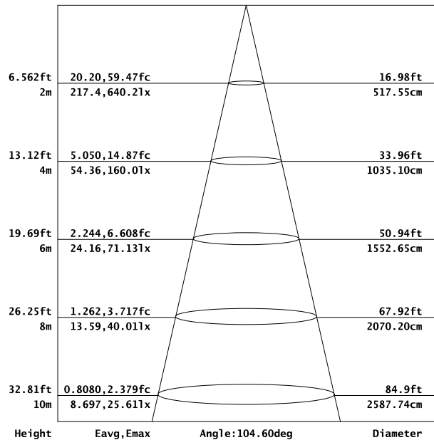
Lux-Distance Curve
